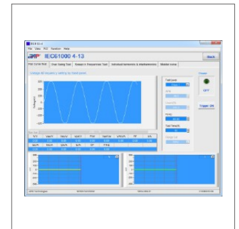
IEC61000 4-13 interface
