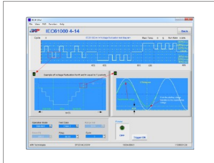
IEC61000 4-14 interface
