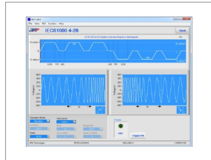
IEC61000 4-28 interface
